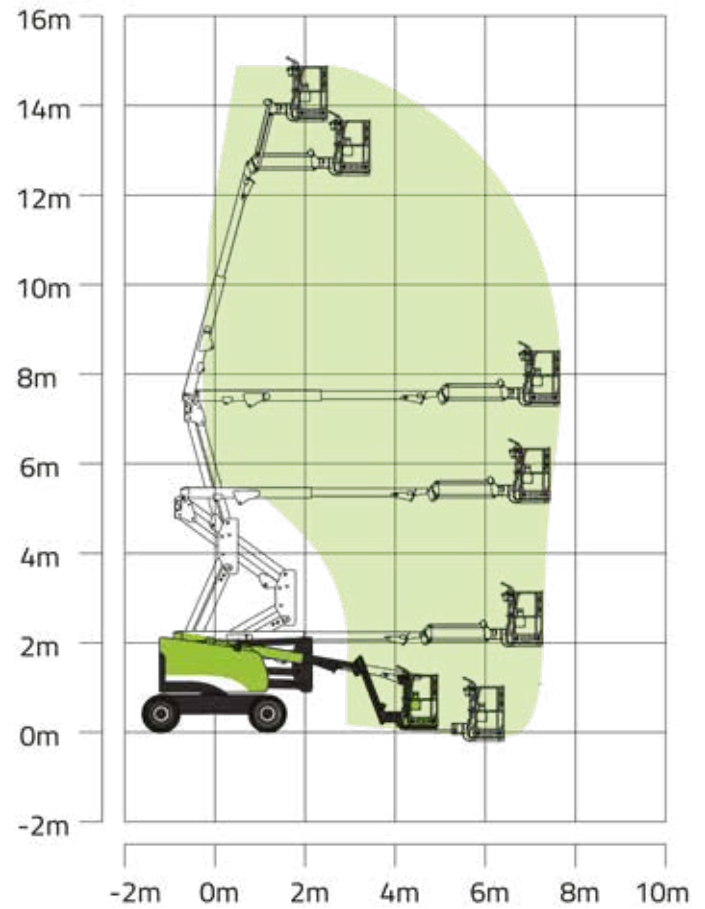
Range of motion ZA14J
