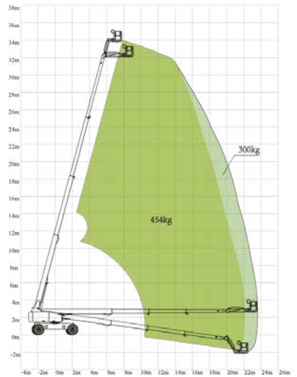
ZT34J Working Envelope
