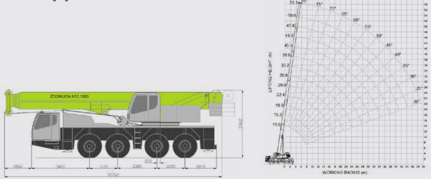
Overall view / Lifting height chart
