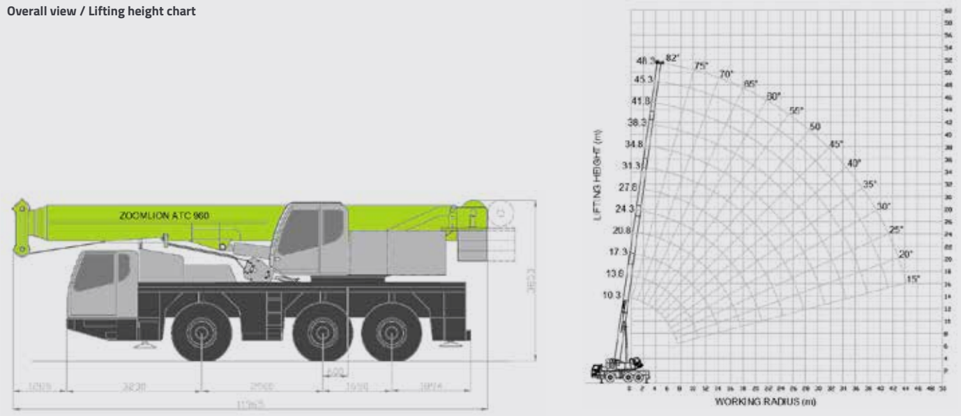
Overall view / Lifting height chart
